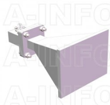
LB-90-15-C-3.5FSP0 Standard Gain Horn Antenna 8.2-12.4GHz 15dB Gain 3.5mm Female
